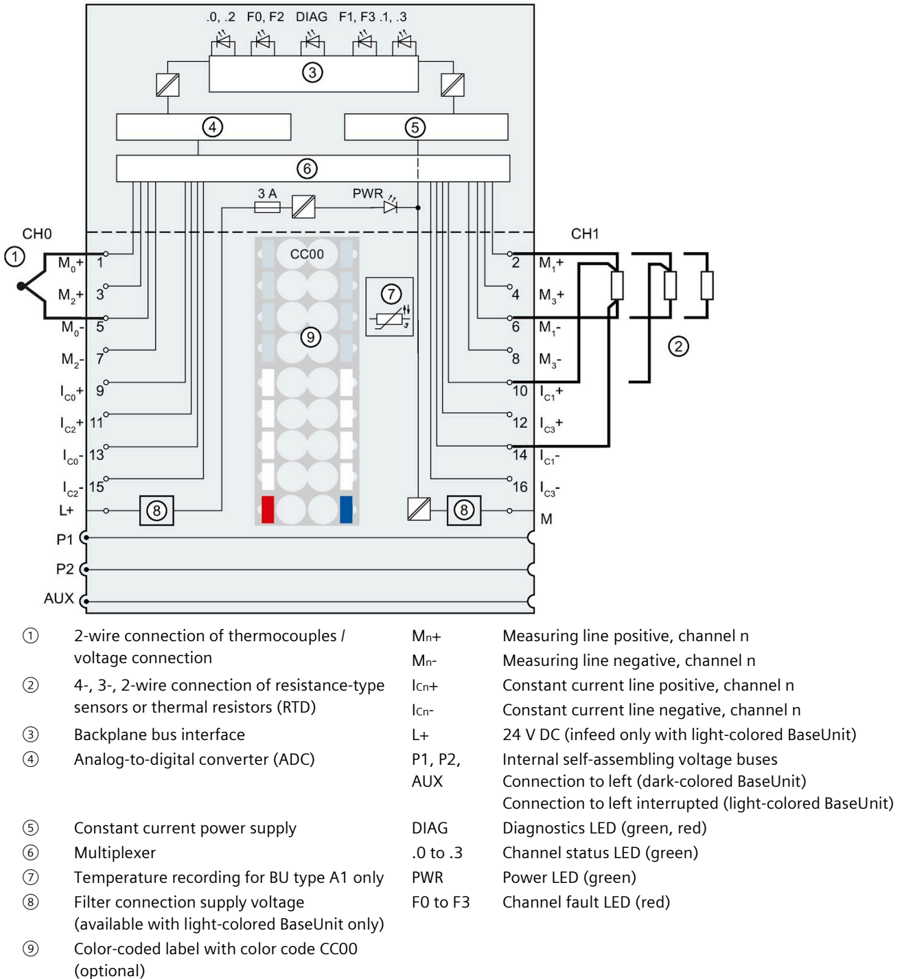
Figure 4-1 Connection and block diagram for connection of thermocouples and resistance-type sensors or thermal resistors (RTD)
