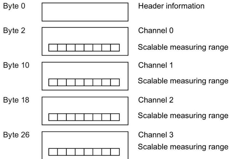
Figure 5-6 Structure of data record 235
