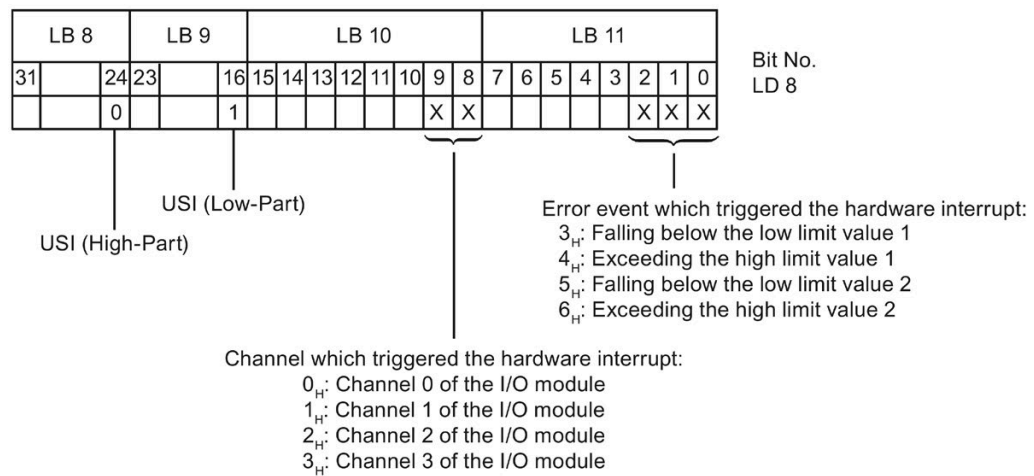
Figure 6-2 OB start information
