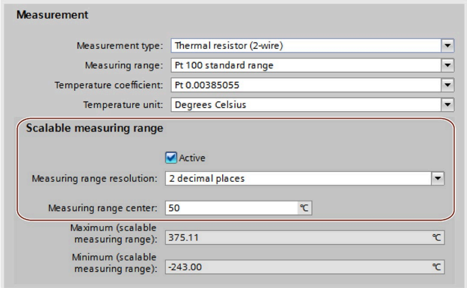
Figure 5-5 Configuration for the scalable measuring range
