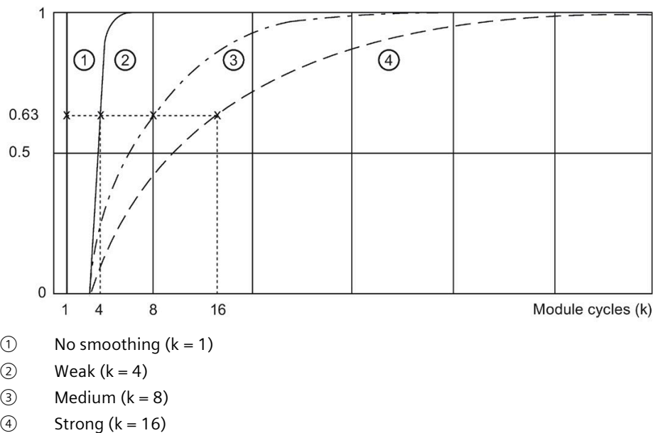
Figure 5-3 Smoothing for AI 4xRTD/TC 2-/3-/4-wire HF
