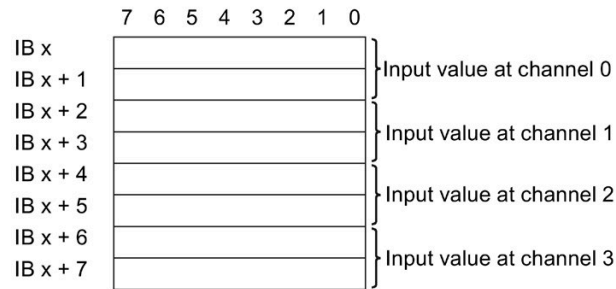
Figure 5-9 Address space AI 4×RTDTC 2-3-4-wire HF without value status
