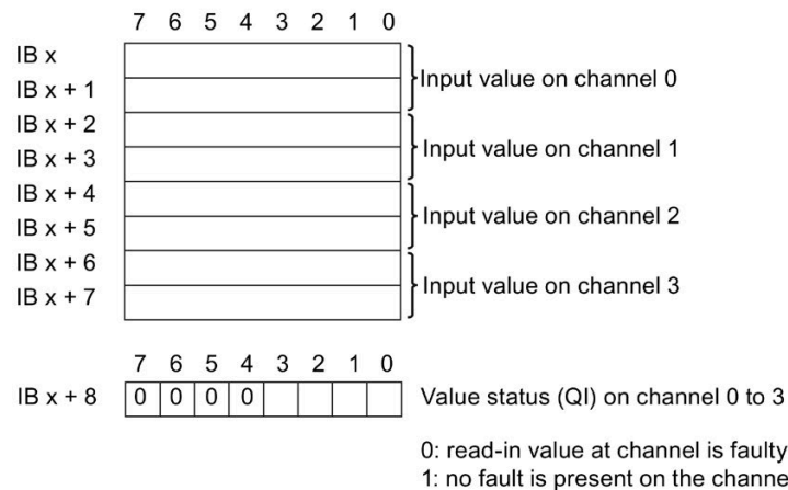
Figure 5-10 Address space AI 4×RTD/TC 2-/3-/4-wire HF with value status
