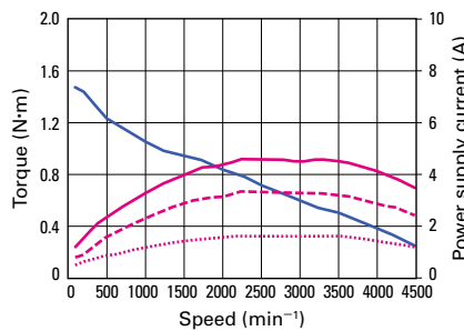
② Motor model number PBM603FCK30-M
