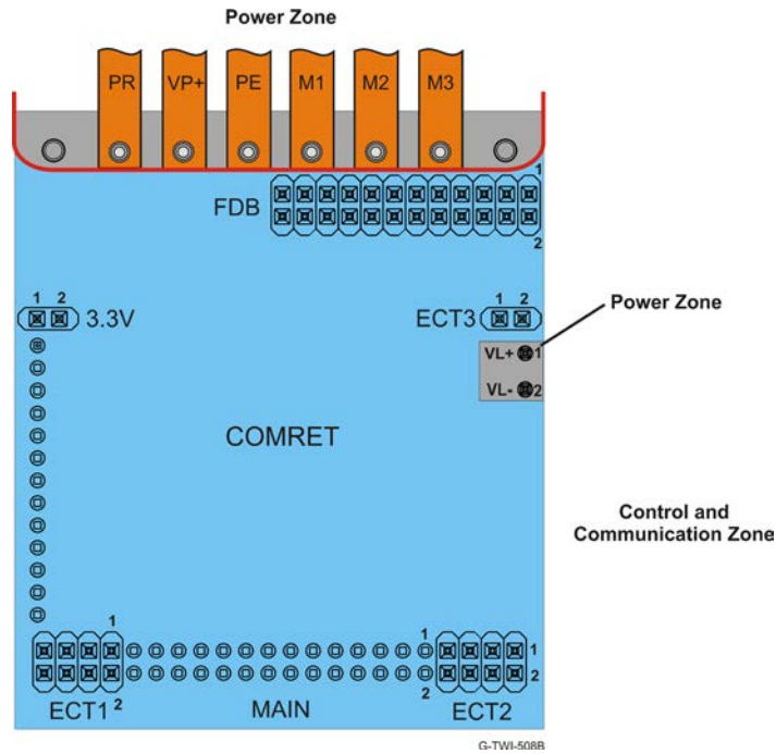
Figure 10: Gold Twitter EtherCAT Power Conductors PCB layout
