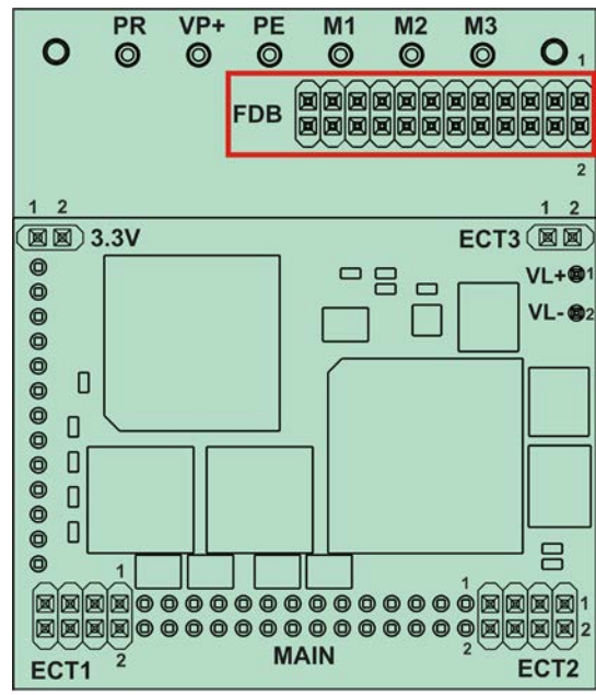
FDB Connector in the EtherCAT option
