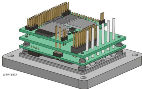
Flat Heat Sink (P/N G-TWIHSFLAT01)
