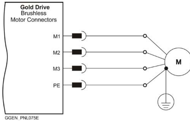
Figure 14: Brushless Motor Power Connection Diagram
