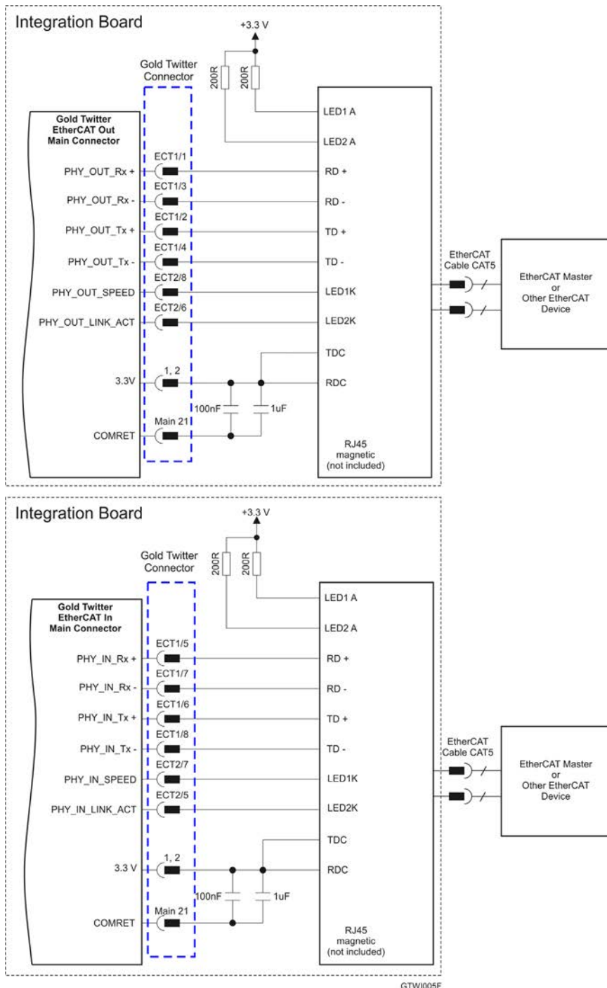
Figure 44: EtherCAT Connection Schematic Diagram
