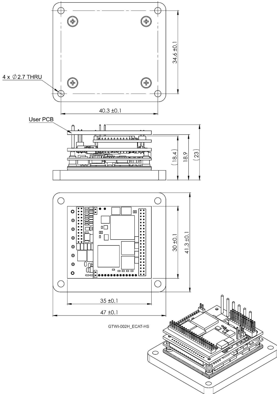
Figure 47: G-Twitter –EtherCAT version
