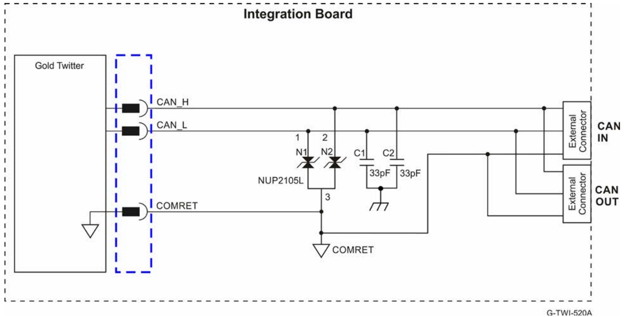
Figure 40: CAN Interface
