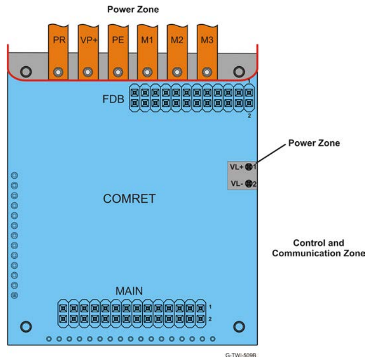
Figure 11: Gold Twitter CAN Power Conductors PCB layout
