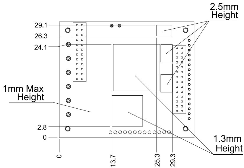
Figure 4: Gold Twitter CAN Version Dimensions3
