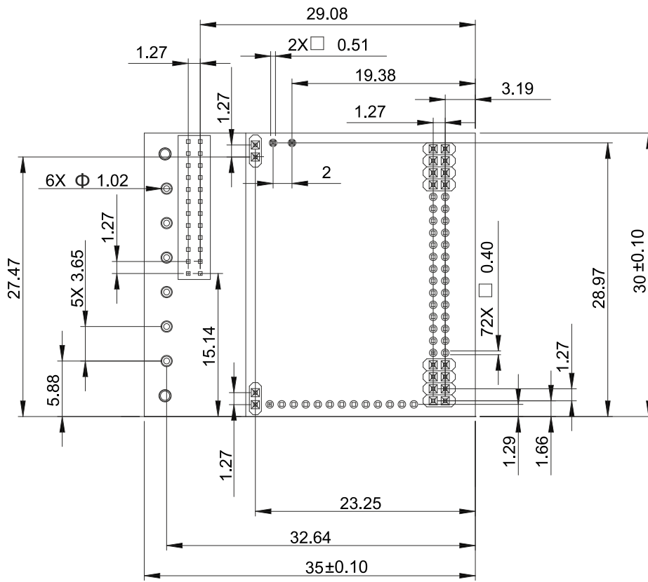
Figure 5: Gold Twitter EtherCAT Version Dimensions
