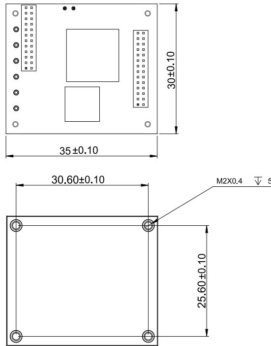
Figure 2: Gold Twitter CAN Version Dimensions1
