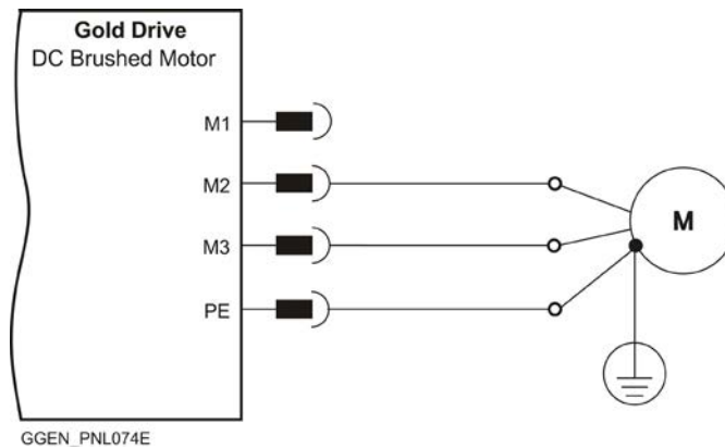
Figure 15: Brushed Motor Power Connection Diagram
