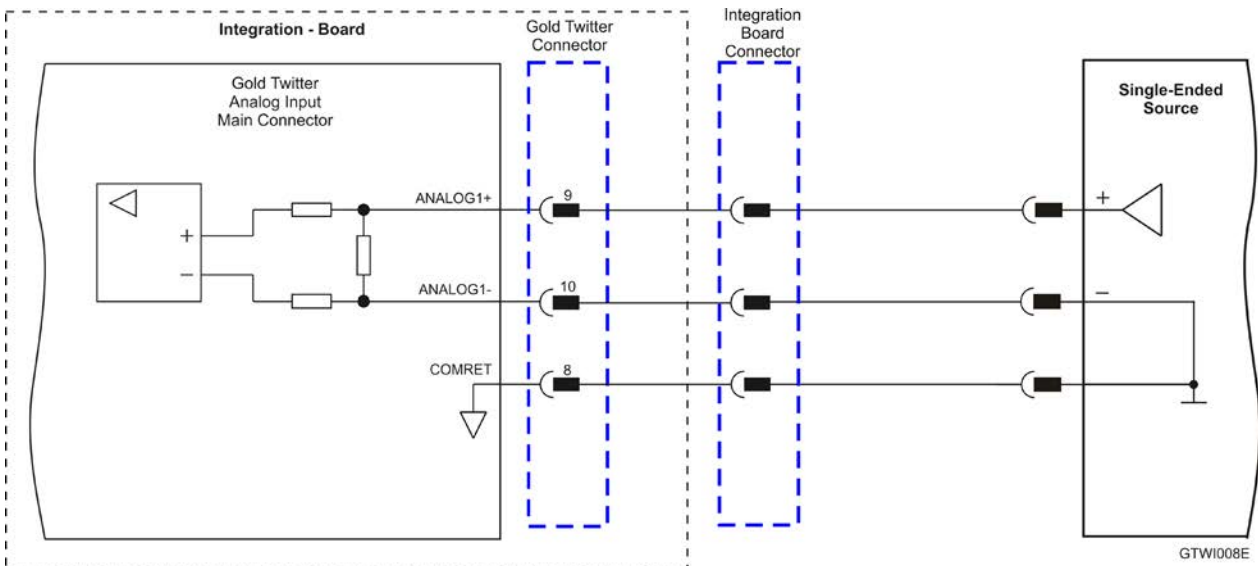
Figure 39: Analog Input
