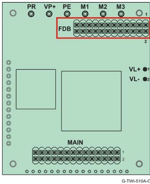
FDB Connector in the CAN option
