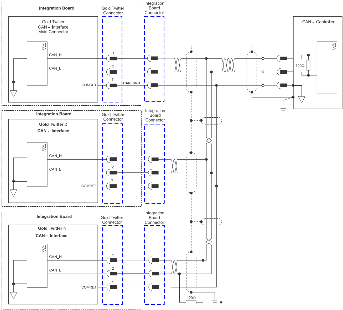
Figure 41: CAN Network Diagram
