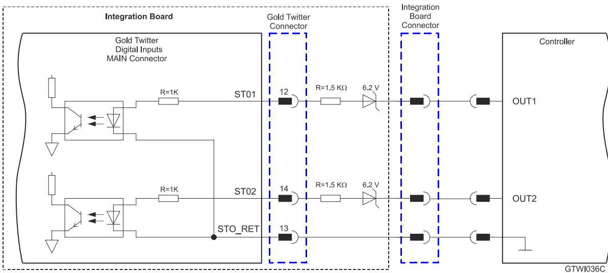
Figure 38: STO Input Connection – PLC (24V Logic)
